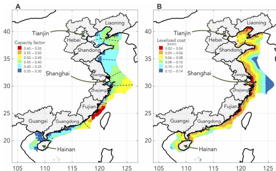
Fig. 1. CFs and levelized costs of electricity. Spatial distributions of the mean (A) CF and (B) LCOE ( \$/\text{kWh}^{-1} ) over 1980–2018 for the filtered region. Coastal provinces are colored gray. The dashed blue lines denote offshore wind areas that are in closest proximity to particular provinces. Note the different color bar limits in (A) and (B).
