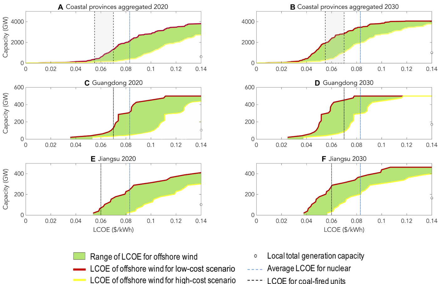
Fig. 2. Offshore wind supply curves. Estimated levelized costs for supply of power from offshore facilities for 2020 (A, C, and E) and 2030 (B, D, and F). The data cover an estimated low-cost (red line) and a potential higher-cost scenario (yellow line). The cost-competitive capacity is defined as the cumulative capacity that could be installed at an LCOE of less than \$0.08 \text{ kWh}^{-1} . For instance, Jiangsu could cost-competitively install roughly 30 GW of offshore wind with the high-cost scenario and roughly 200 GW in the low-cost scenario assuming costs that would apply currently in 2020.
